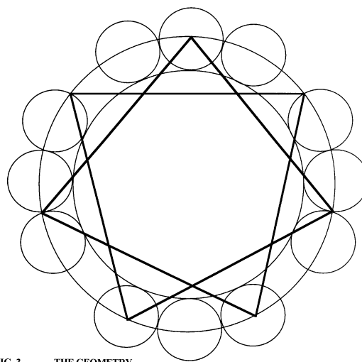
FIG. 3 THE GEOMETRY
